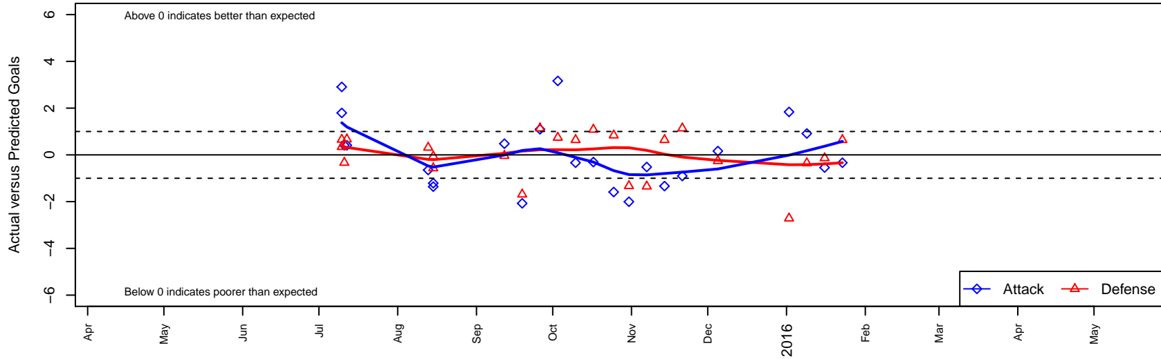
Lake Hills Supreme G02 Dots are actual minus expected GF (blue circles) and GA (red triangles). Blue line is smoothed change in attack strength. Red is smoothed change in defense strength.
